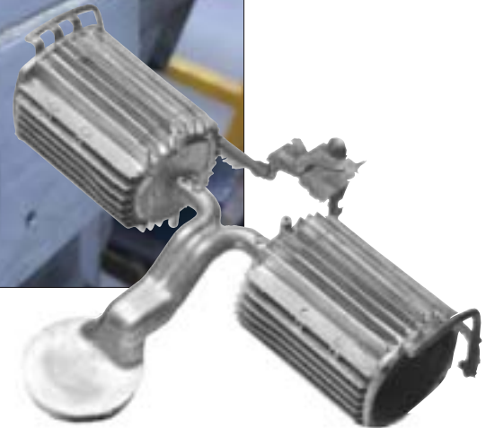
Aluminium pump housing fixed to the filling system, i.e. runners, gates and overflows.
